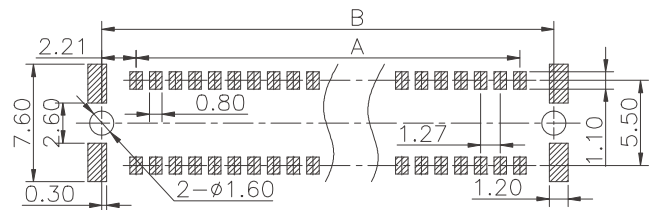
Recommended P.C.Board Layout (Tolerance: \pm 0.05 )
