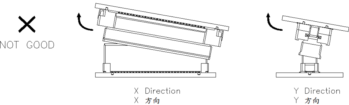
Figure-5 Withdrawal with an angle 图5 带角度的拔出
