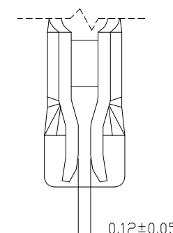
DETAIL: C SCALE 2: 1
