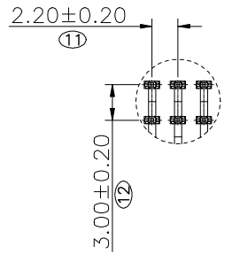
DETAIL G SCALE 2:1
