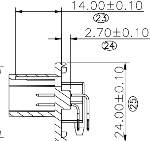
SECTION F-F
