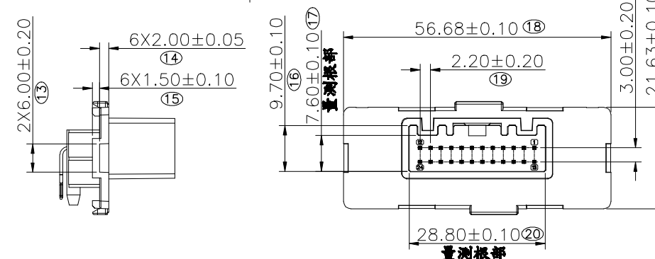
SECTION F-F
