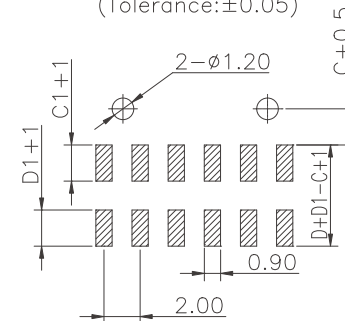
Recommended P.C.Board Layout (Tolerance:±0.05)
