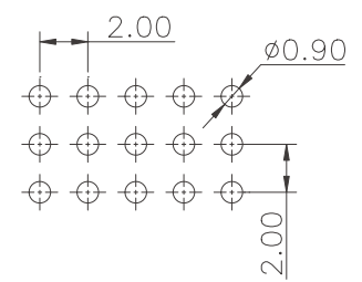
Recommended P.C.Board Layout (Tolerance:±0.05)
