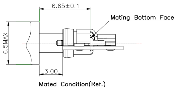
Mated Condition(Ref.)
