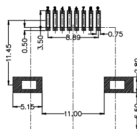
RECOMMENDED PCB LAYOUT VIEWED FROM COMPONENT SIDE
