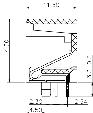
CUTAWAY VIEW
