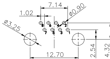
PCB LAYOUT (±0.05)
