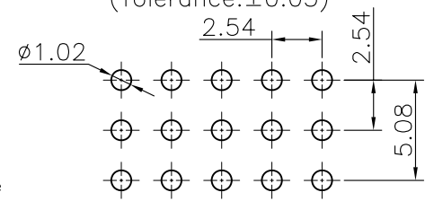
Recommended P.C.Board Layout (Tolerance:±0.05)
