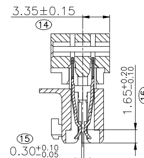
SECTION F-F
