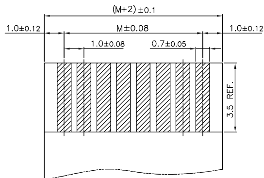
适用FPC尺寸 APPLICABLE FPC
