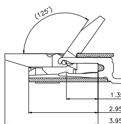
SECTION A-A(2:1)
