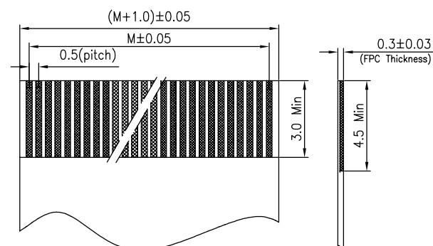
適用FPC尺法 APPLICABLE FPC
