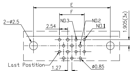
PCB Layout (14,26,50 Pos)
