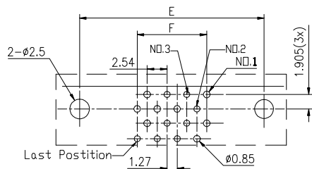
PCB Layout (20,36,40,68,100 Pos)
